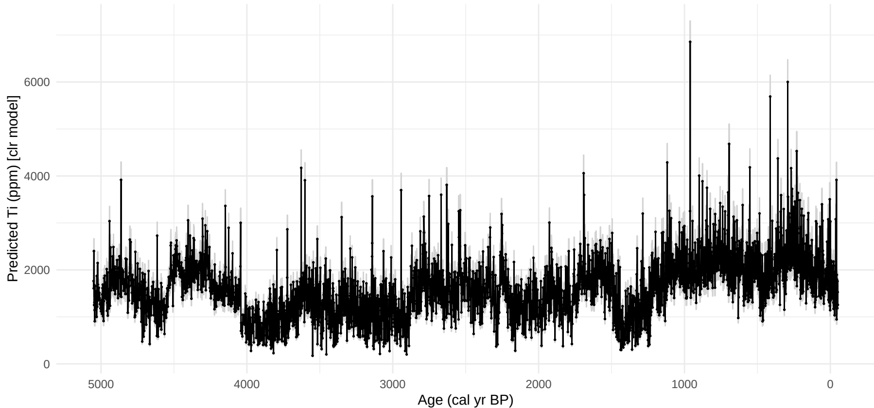
HER42PB: PLSR Ti Predictions with Confidence Interval (clr model)
